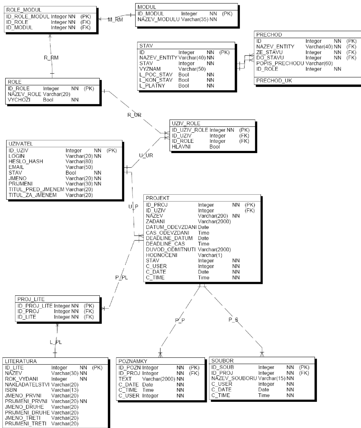
Obr. 5.1 E-R model
