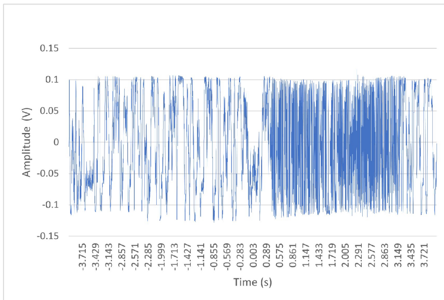
Fig. 7.2: Knocking on the hard surface near the sensing cable
