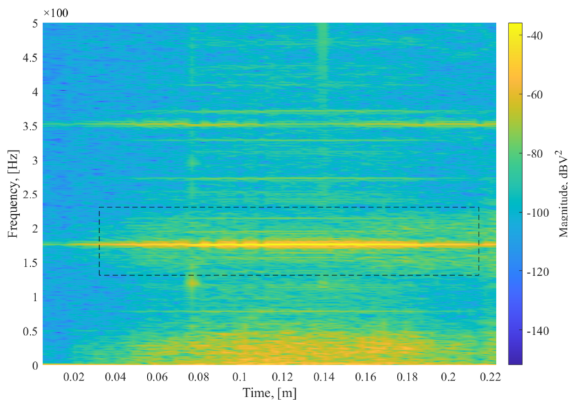
Fig. 7.9: Spectrogram of walking
