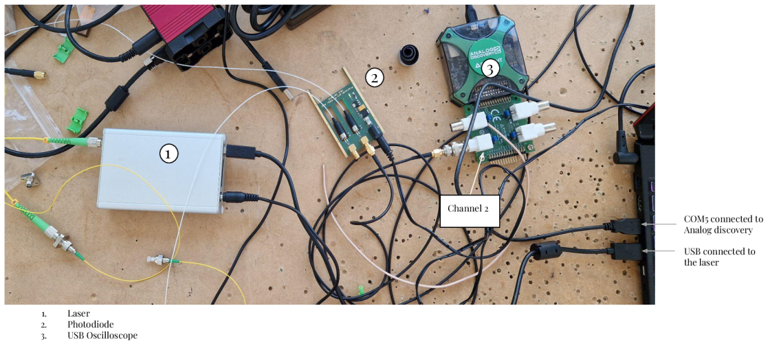
Fig. 7.7: Connection to the control unit
