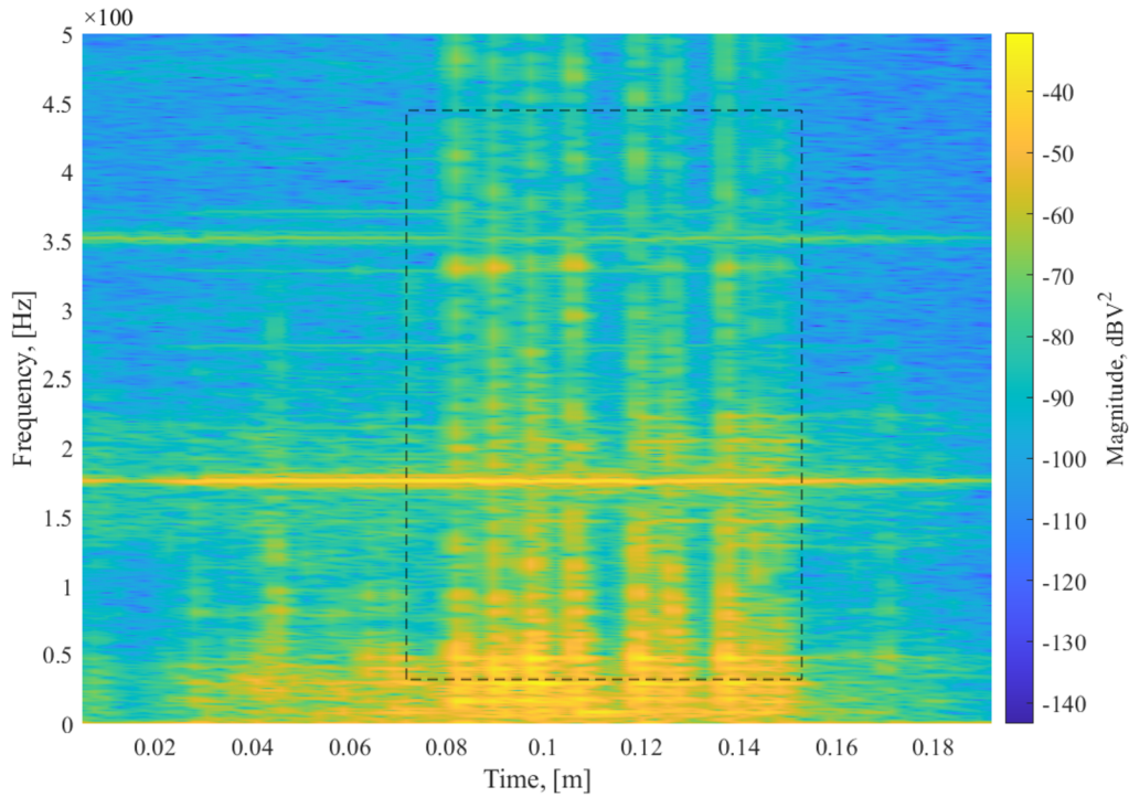
Fig. 7.11: Spectrogram of stomping
