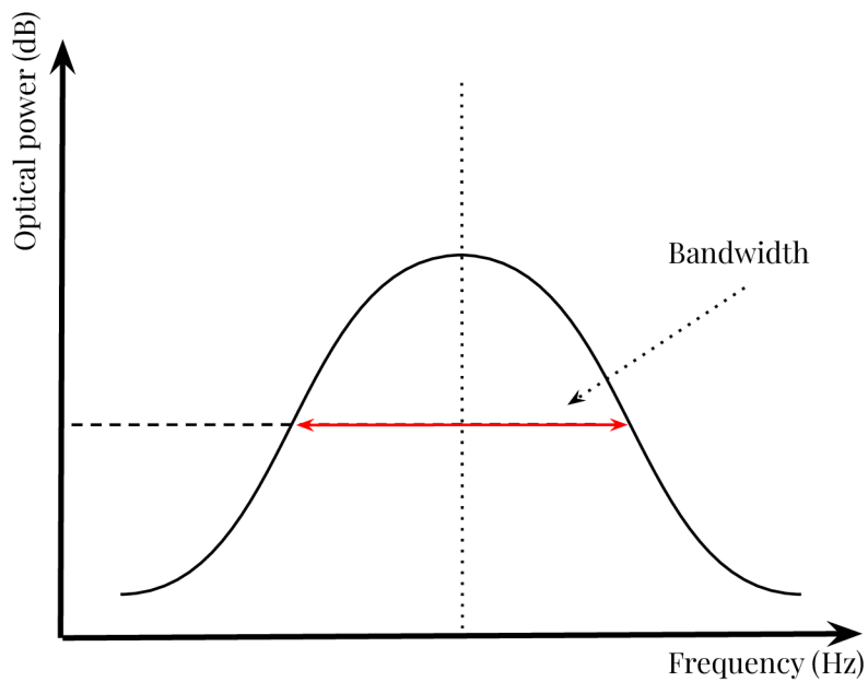
Fig. 1.3: Bandwidth [43]
