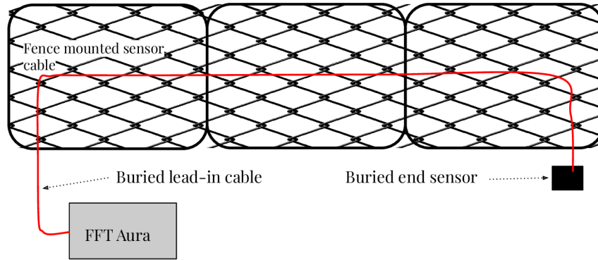
Fig. 6.1: Future Fiber Technology Aura system deployment [30]
