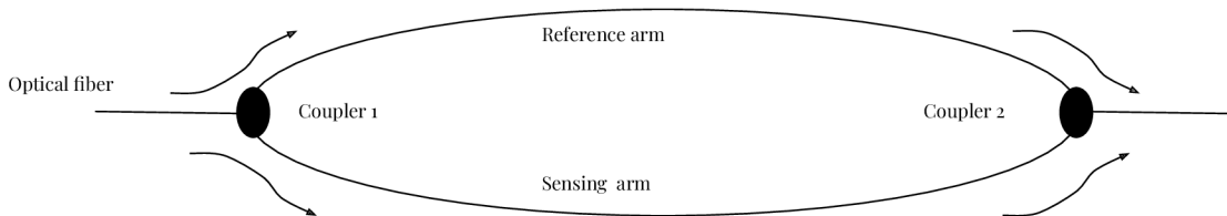
Fig. 5.2: Mach-Zender Optical Interferometer construction [21]
