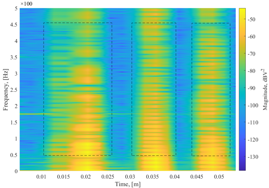
Fig. 7.13: Spectrogram representing jumping
