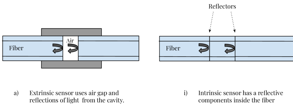
Fig. 5.1: Fabry-Perot Optical Interferometer construction [21]
