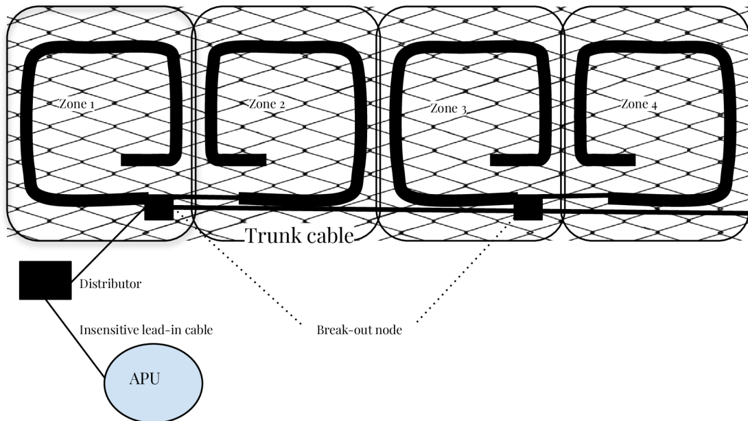
Fig. 5.5: Fiber Defender system deployment [25]
