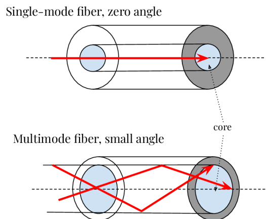
Fig. 2.2: Light propagation in the fiber [2], [9]
