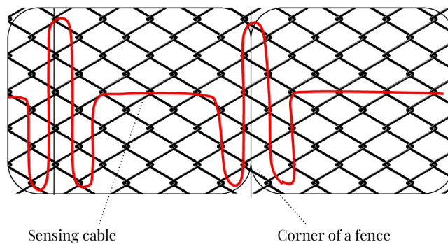
Fig. 6.2: Future Fiber Technology Aura system deployment around the corners[30]
