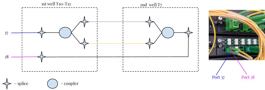
Fig. 7.6: Mach-zender interferometer-based system for the practical section
