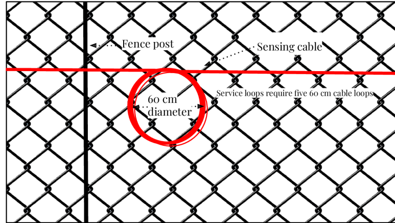
Fig. 6.3: Fiber Patrol service loops installation[32]
