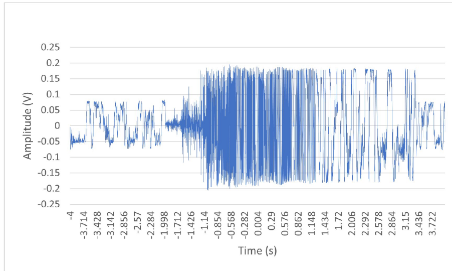
Fig. 7.3: Interfering with the sensing cable directly
