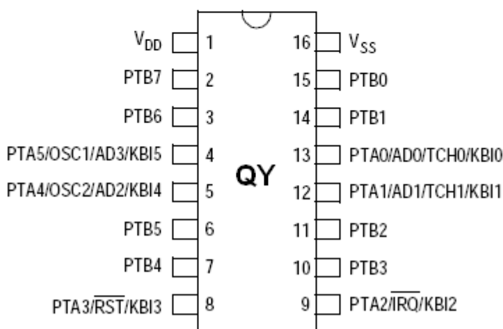
MC68HC908QY4
