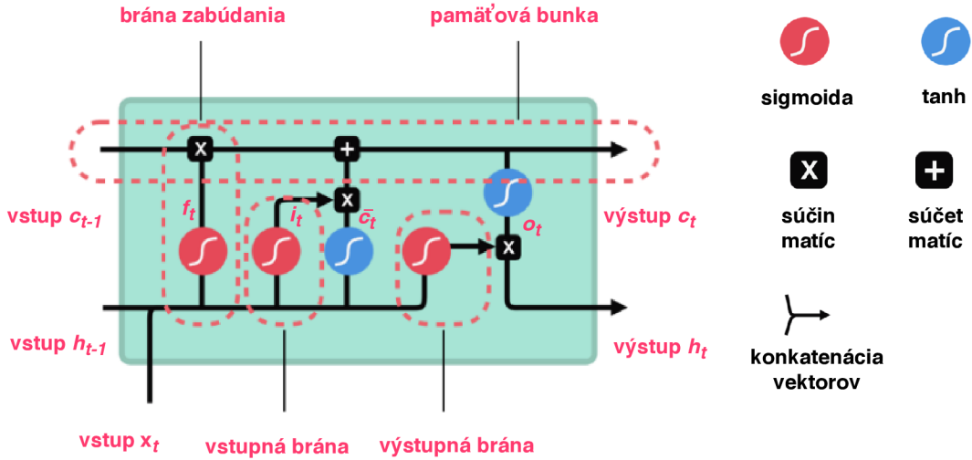
Obr. 3.7: Schéma LSTM [25]
