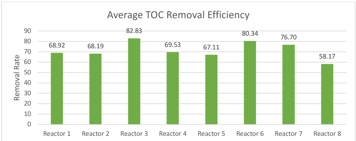
Figure 5.6.2: Average removal efficiency for Total Organic Carbon
