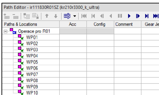
Obr. 45 – Path Editor
