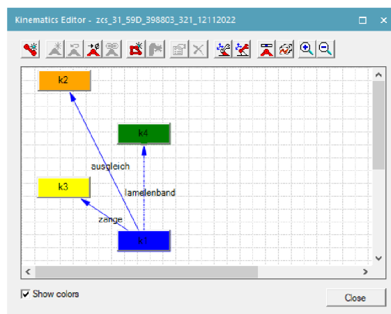
Obr. 29 – Kinematic Editor 2
