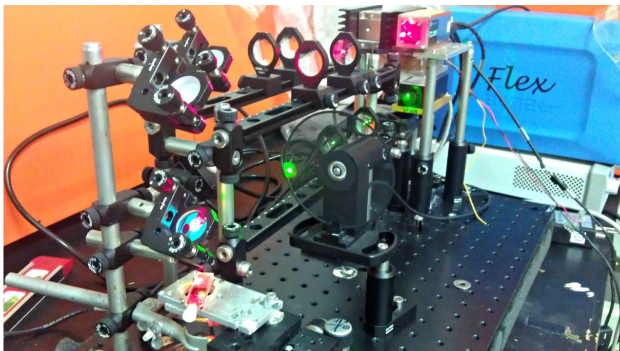
Figure 33. TLM system
