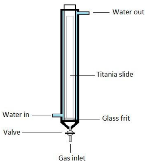
Figure 19. Scheme of the reactor cell.
