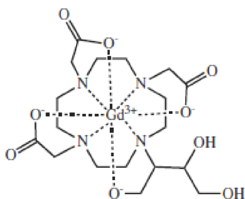
Gd-BT-DO3A (Gadovist®)
