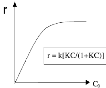
Figure 6. Influence of initial concentration C_0 on photocatalytic reaction rate r . [16]
