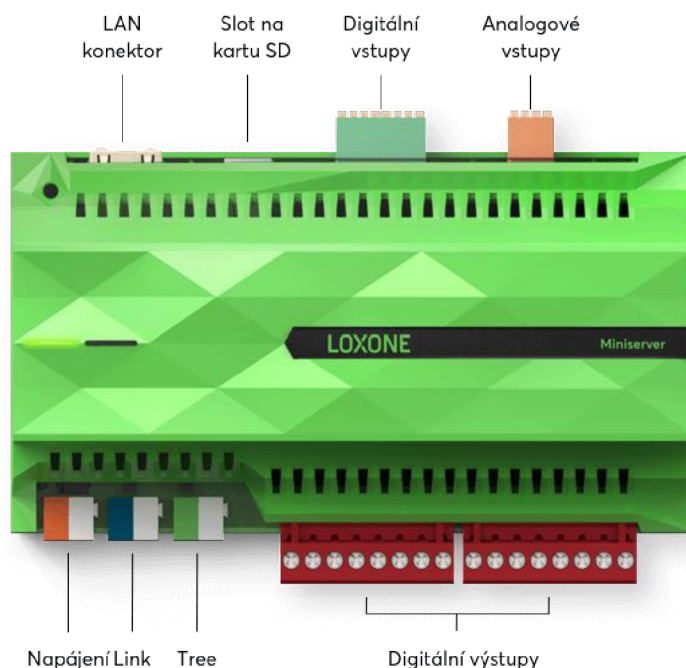
Obr. 8: Loxone Miniserver [11]
