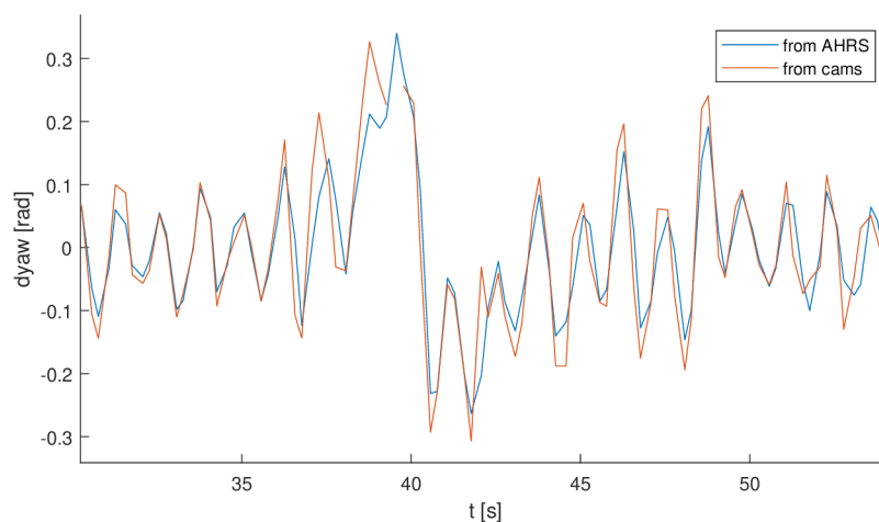
Figure 6.7: Comparison of heading change extracted from AHRS and front/back cameras.
