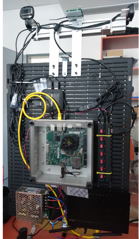
Figure 5.4: Second-generation wearable platform, rear view.
