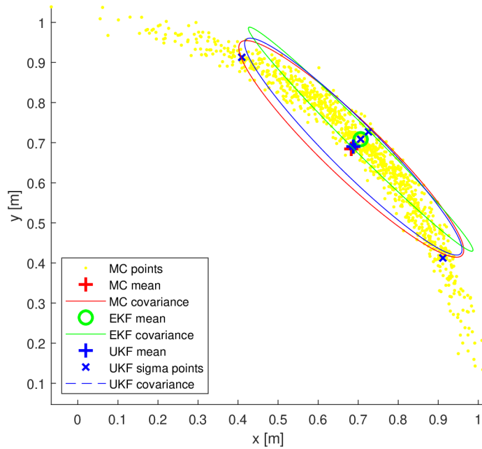
Figure 3.6: Comparison of mean and covariance estimation through 1000-samples Monte Carlo as ground truth, EKF and UKF mechanisms. The non-linear function is a simple distance/bearing beacon model given by [x; y] = [r \cos(\phi); r \sin(\phi)] ; true covariance of the r and \phi inputs is P = [0.0004 \ 0; 0 \ 0.068] . Covariance ellipses denote 68% confidence interval.
