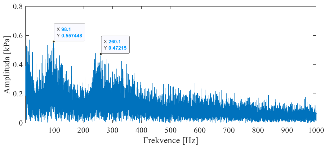
Obr. 8.6 – FFT, \sigma = 0,217
