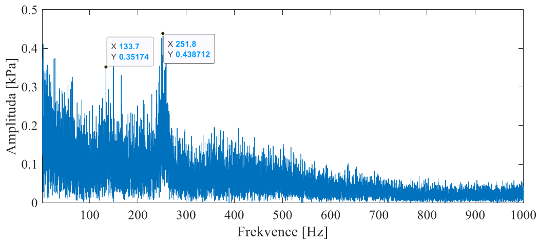
Obr. 8.4 – FFT, \sigma = 0,282
