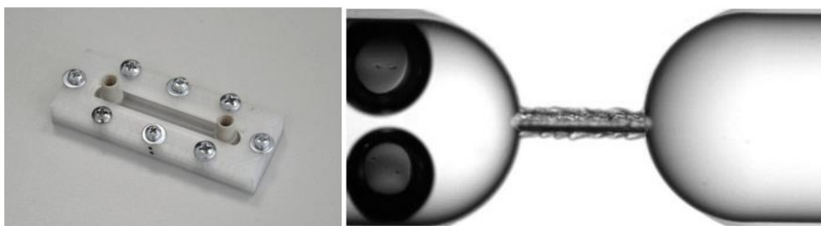
Obr. 3.1 – Sestava čipu a detail clonky [25]
