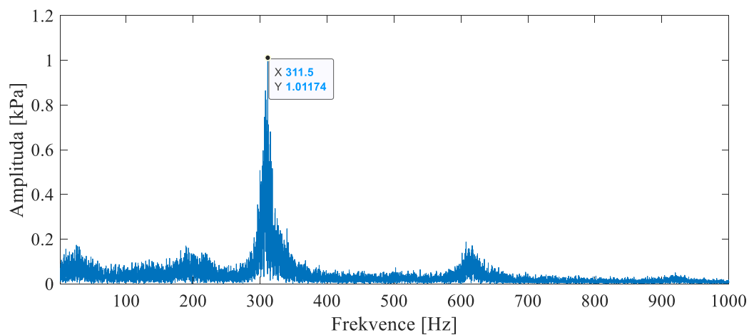
Obr. 8.2 – FFT, \sigma = 0,403
