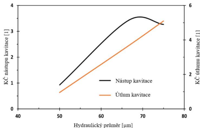
Obr. 2.8 – Hystereze [20]
