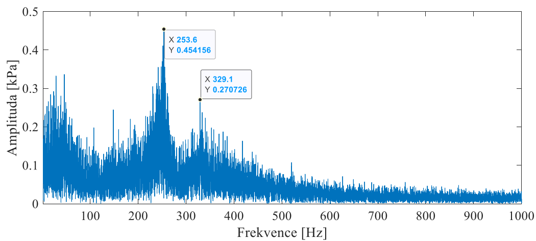
Obr. 8.3 – FFT, \sigma = 0,322
