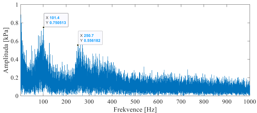
Obr. 8.7 – FFT, \sigma = 0,197
