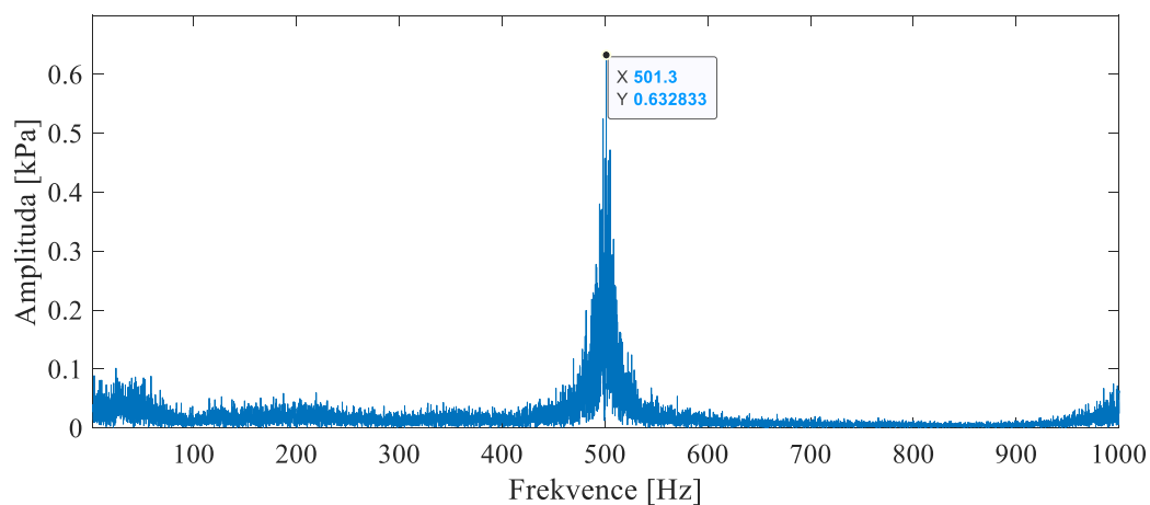
Obr. 8.1 – FFT, \sigma = 0,528
