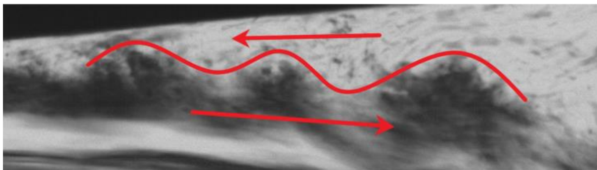
Obr. 4.15 – Vznik Kelvin-Helmholtzovy nestability, \sigma = 0,144
