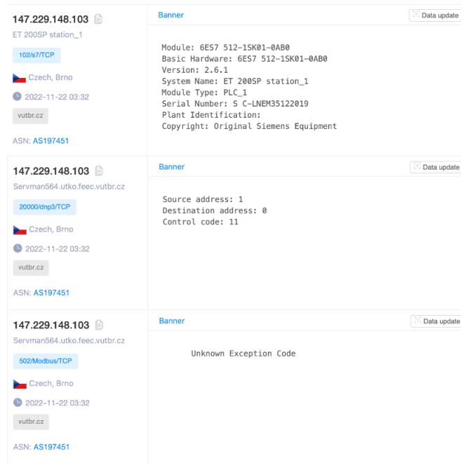
Fig. 3.3: ZoomEye results
