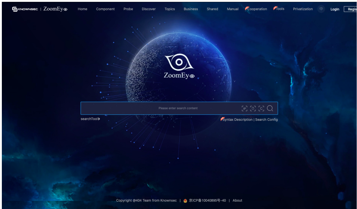
Fig. 2.6: ZoomEye homepage
