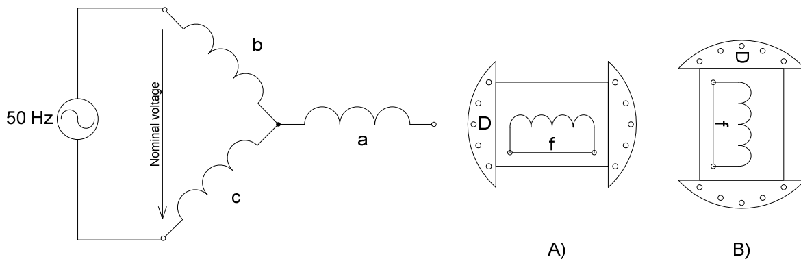
Fig. 31- Setup for Single Frequency Response Test for: A) d axis subtransient reactance B) q axis subtransient reactance
