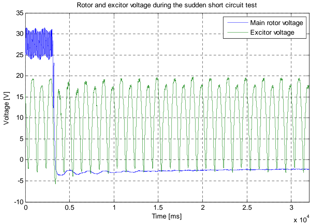
Fig. 42- Rotor and excitor voltage during the sudden short circuit test
