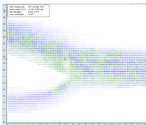
Obr. 21 Vector Statistics
