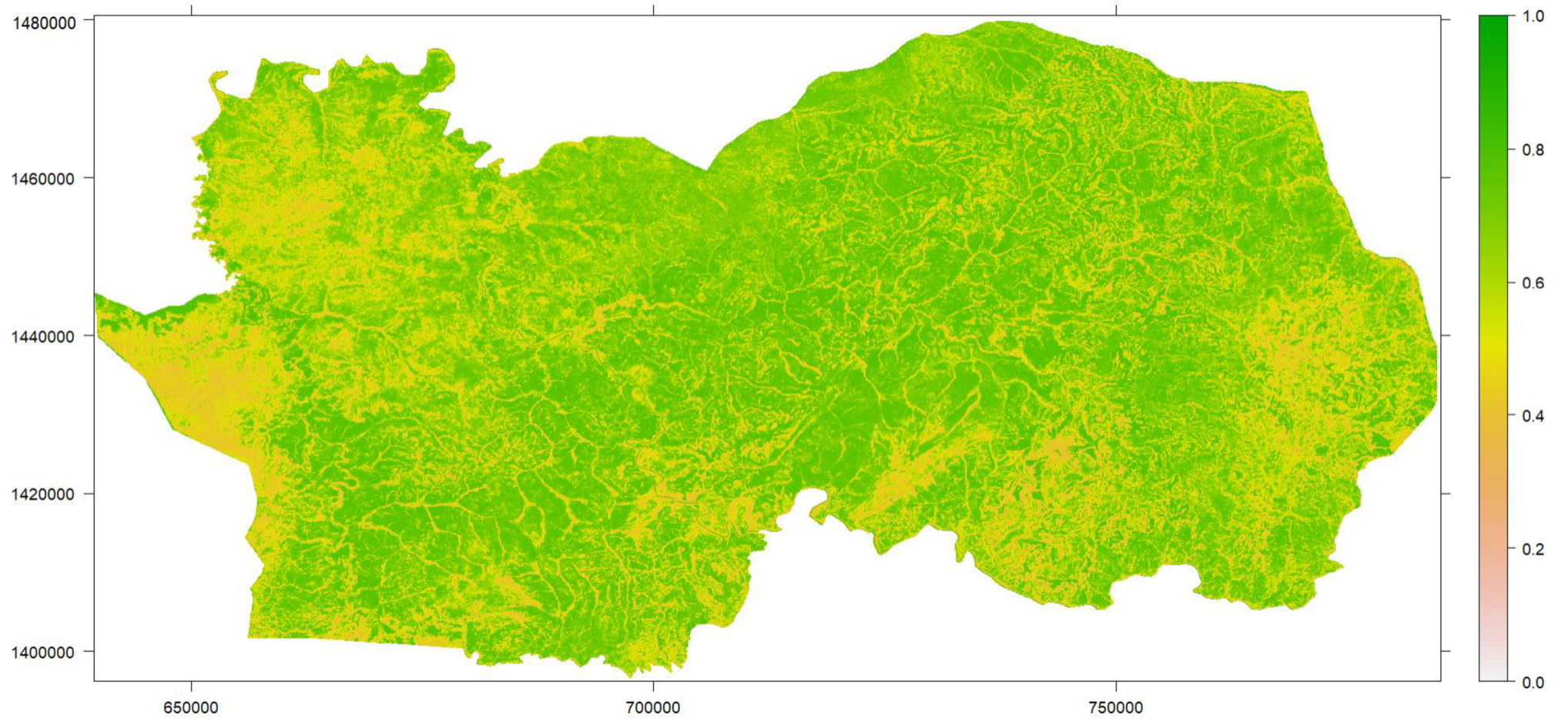
Figure 16: Prediction map of the probability of Roan occurrence/presence in NKNP
