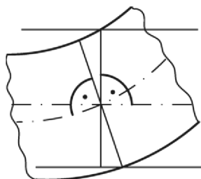
Obr. 4.12 Deformace prutu [5]
