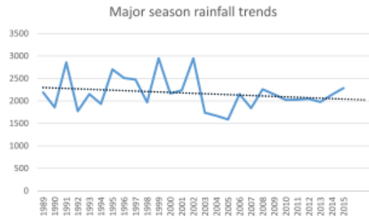
Figure 3a. Rainfall trend for the major raining season
