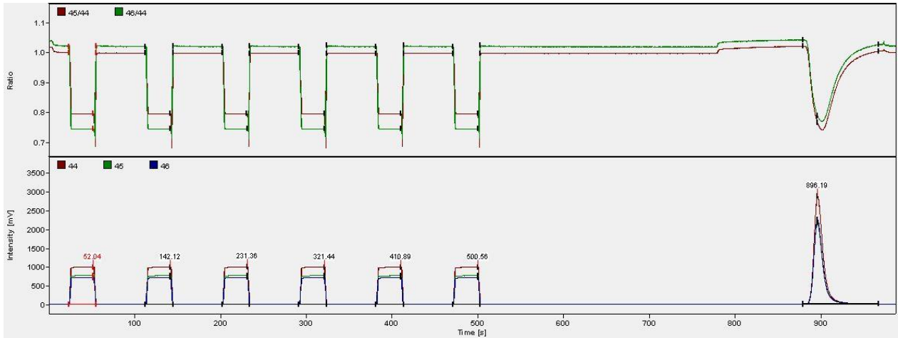
Figure 4: Example of an isotope ratio (upper) and mass trace chromatogram (lower) of N_2O converted from an in-house potassium nitrate standard and detected by the IRMS. The first six box-shaped peaks are pulses of the N_2O working gas; the peak on the far right is N_2O converted from NO_3^- .
