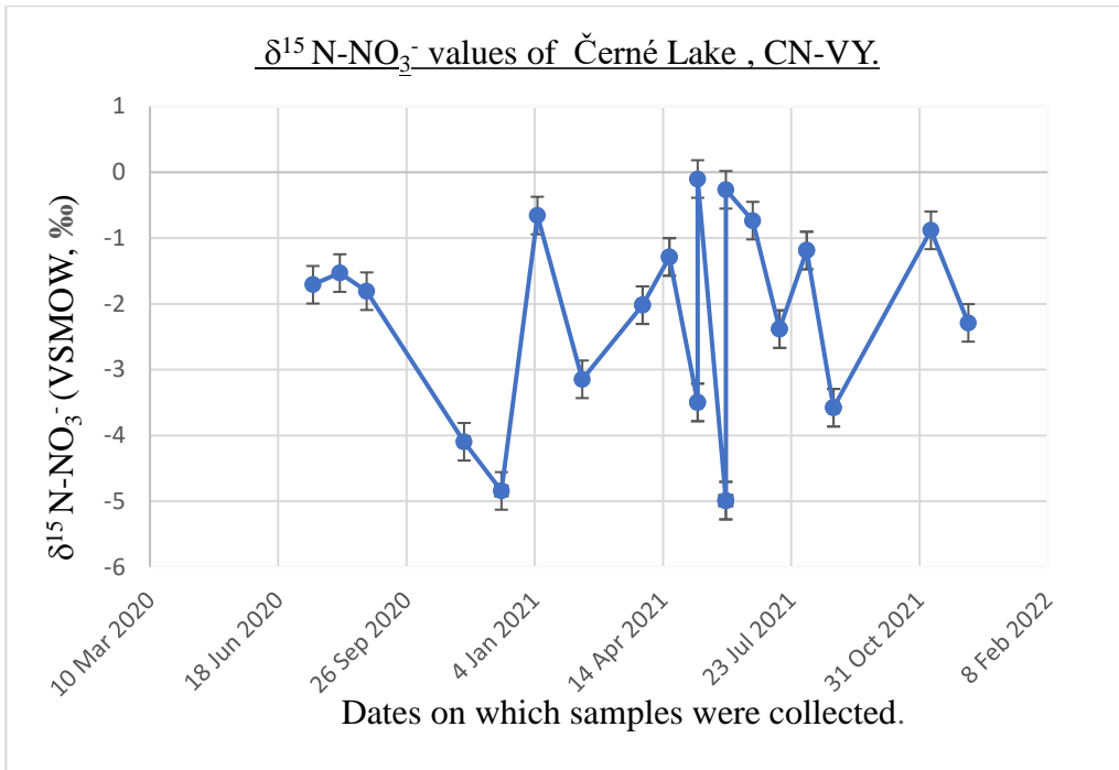
Figure 15: shows the \delta^{15}\text{N-NO}_3^- in Černe Lake outlet, CN-VY.
