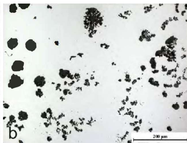
Obr. 7: Chunky grafit [13].
