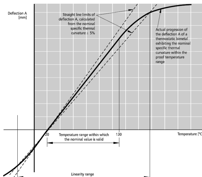
Obr. 11: Rozmezí linearity [2]
