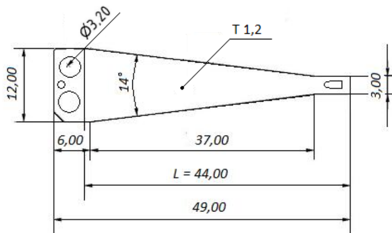
Obr. 24: Geometrie bimetalu [1]
