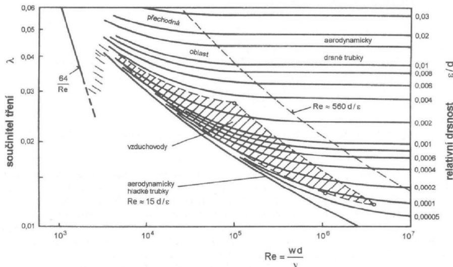
Obr. 3.7 – Moodyho diagram [34]
