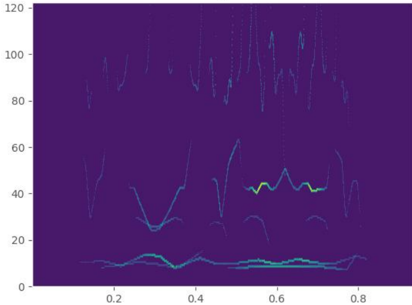
Figure 5.12: IMFogram generated from the IMFs of the anti-symmetric and symmetric extension
