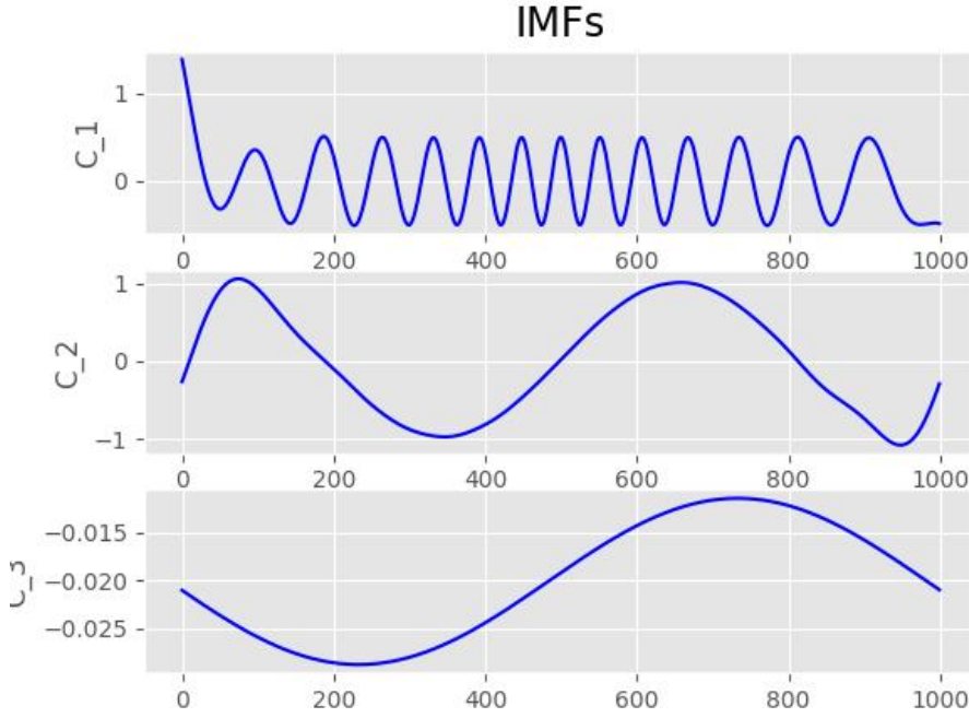
Figure 2.2: The IMFs of the artificial signal S(t)
