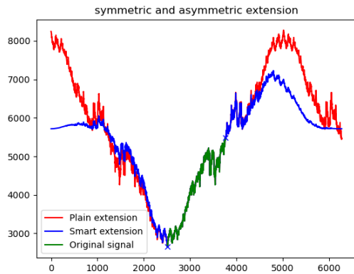
Figure 5.13: Asymmetric and Symmetric extension of Nasdaq
