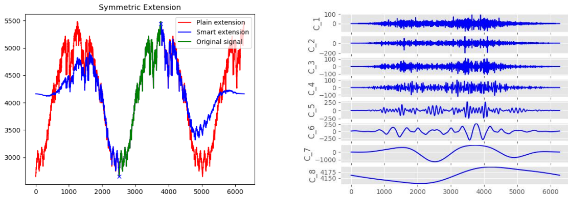
Figure 5.7: symmetric extension of Nasdaq Figure 5.8: IMFs of the symmetric extension
