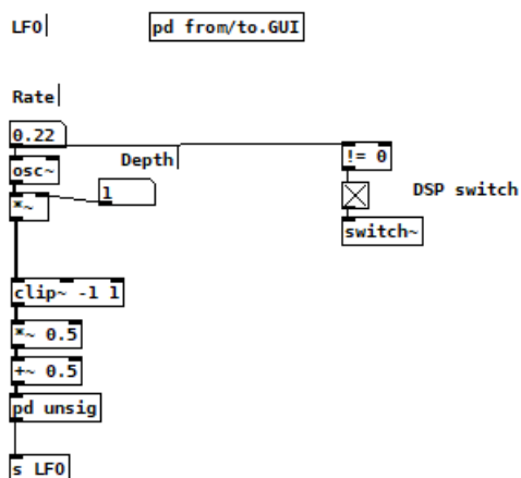
Obr. 3.16: Subpatch LFO
