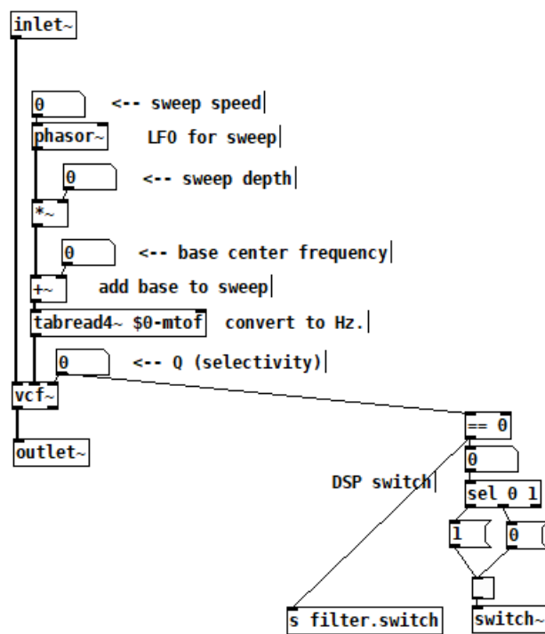
Obr. 3.17: Filter
