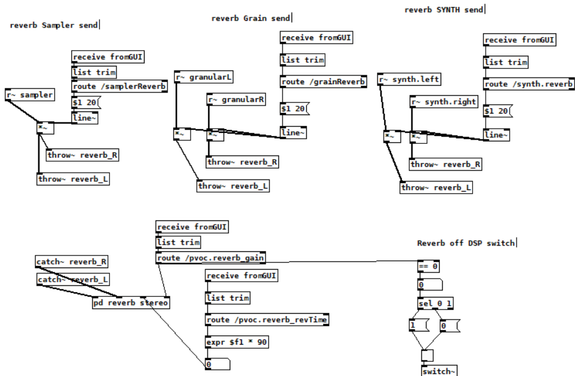
Obr. 3.18: Efekt reverb
