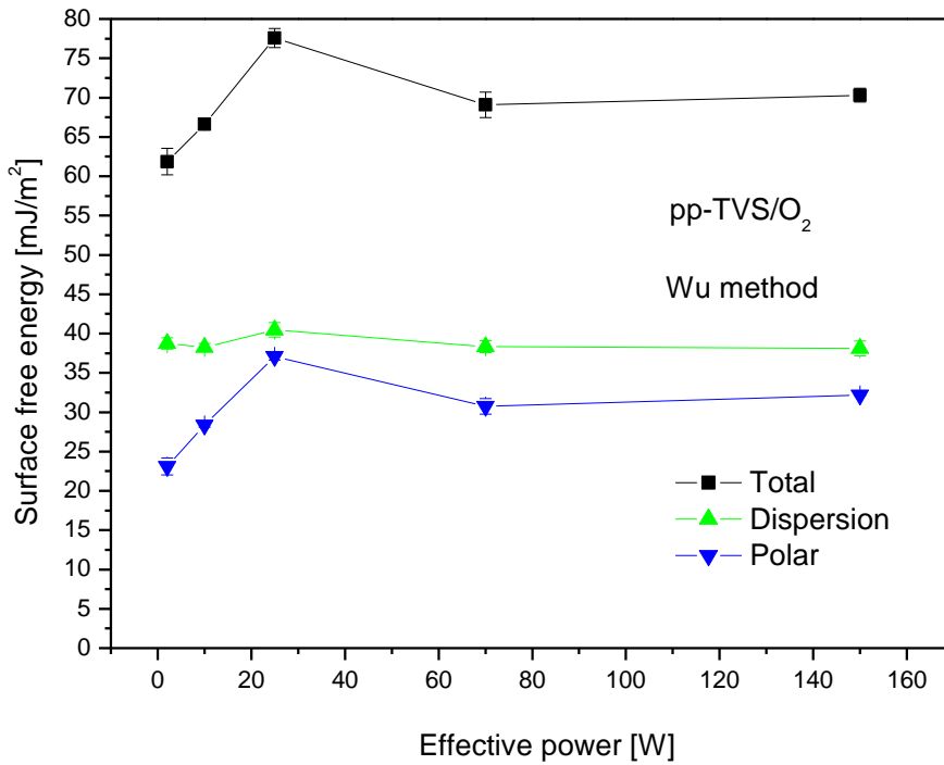
Fig. 25: Wu method components dependence of pp-TVS/O₂
